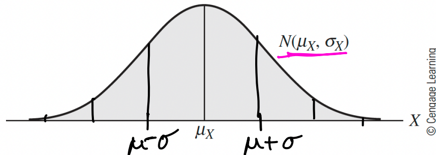
FIGURE 3.4 A normal distribution
