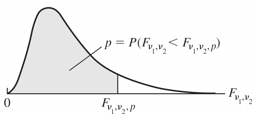
(c) F distribution
