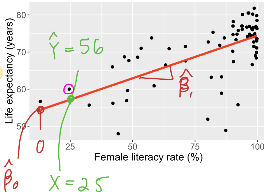
Relationship between life expectancy and the female literacy rate in 2011
